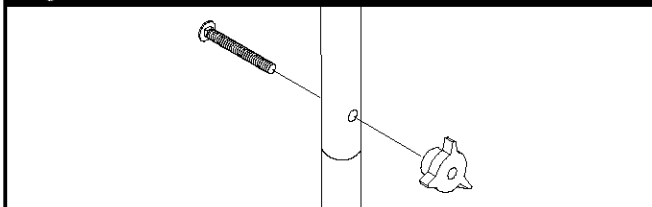
Figure 4 — Secure Handle
